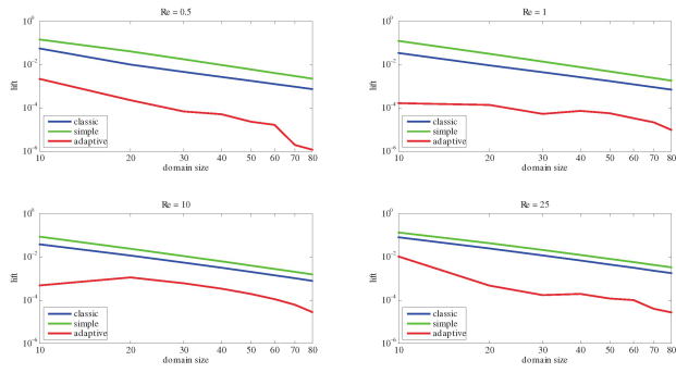
Figure 2: Error on lift.
