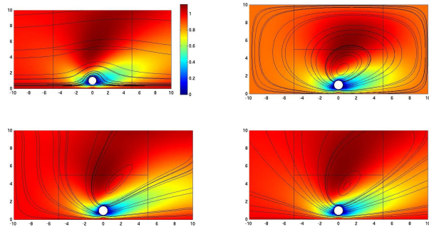
Figure 3: Qualitative behavior based on b.c. type.
